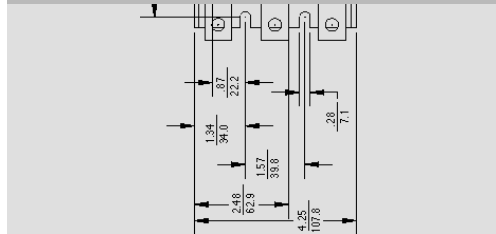
RT3 - Front View
